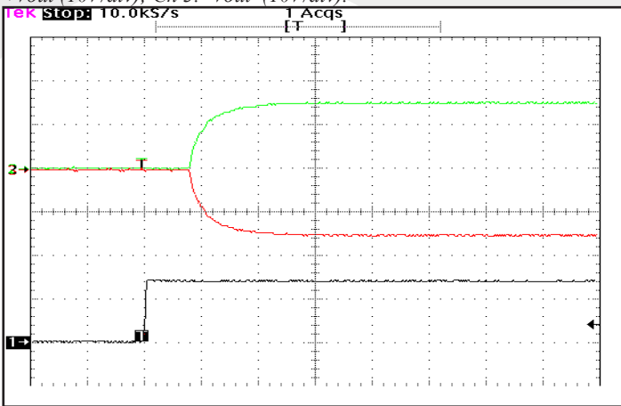
Figure 15: Turn-on transient at full load current, after application of input voltage (ENA 1 logic high) (5ms/div). Input voltage pre-applied. Ch 1: Enable1 input (20V/div); Ch 2: +Vout (10V/div); Ch 3: -Vout (10V/div).
