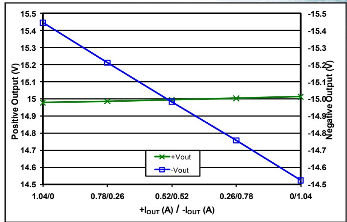
Figure 8: Load regulation vs. load current with power fixed at 80% load (16W) and load currents split as shown between the +15V and -15V outputs, at nominal input voltage and T case = 25°C.
