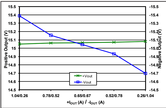
Figure 7: Load regulation vs. load current with power fixed at full load (20W) and load currents split as shown between the +15V and -15V outputs, at nominal input voltage and T case = 25°C.
