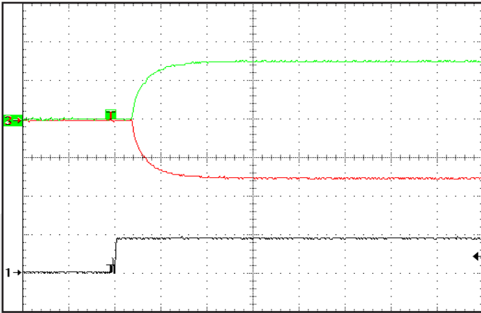
Figure 13: Turn-on transient at full load current (resistive load) (5 ms/div). Input voltage pre-applied. Ch 1: Enable1 input (5V/div); Ch 2: +Vout (10V/div); Ch 3: -Vout (10V/div).
