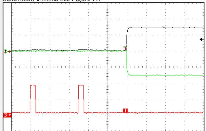
Figure 22: Rise of output voltage after the removal of a short across the positive output terminals. Ch 1: +V_{out} (10V/div); Ch 2: -V_{out} (10V/div); Ch 3: +I_{out} (1A/div).
