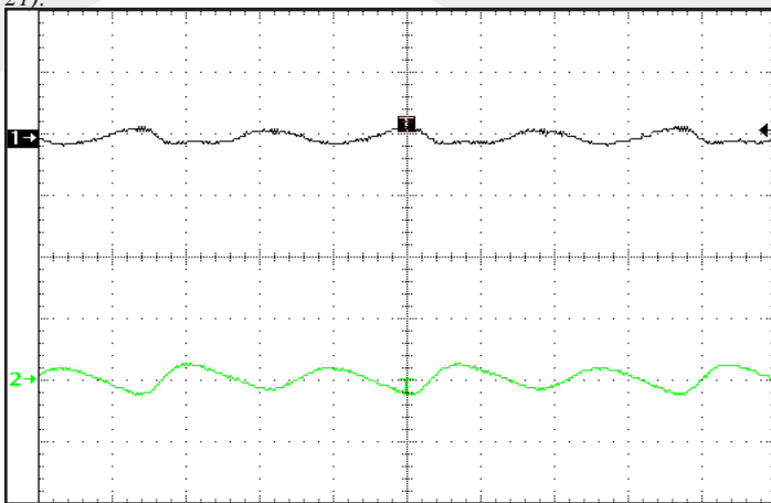
Figure 21: Output voltage ripple, +V_{out} (Ch 1) and -V_{out} (Ch 2), at nominal input voltage and full load current evenly split (50mV/div). Load capacitance: 1\ \mu\text{F} ceramic cap and 10\ \mu\text{F} tantalum cap.. Bandwidth; 10MHz. See Figure 19.
