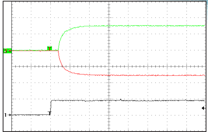
Figure 14: Turn-on transient at zero load current (5ms/div). Input voltage pre-applied. Ch 1: Enable1 input (5V/div); Ch 2: +Vout (10V/div); Ch 3: -Vout (10V/div).
