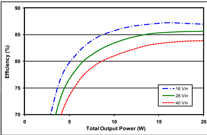
Figure 1: Efficiency vs. output power, from zero load to full load with equal load on the +15V and -15V outputs at minimum, nominal, and maximum input voltage at Tcase=25°C.
